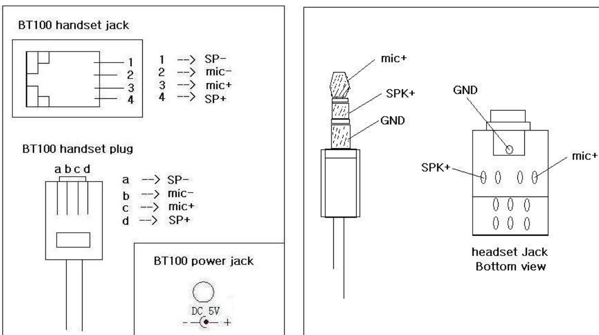
Figure 2: GXP-2000 Internal Headset Wiring Schema
